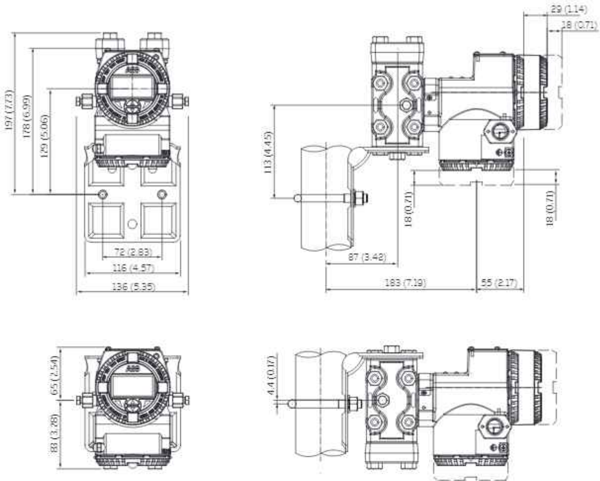
Figure 5 Transmitter with DIN aluminum housing - horizontal flanges on bracket for vertical or horizontal 60 mm. (2 in.) pipe mounting
