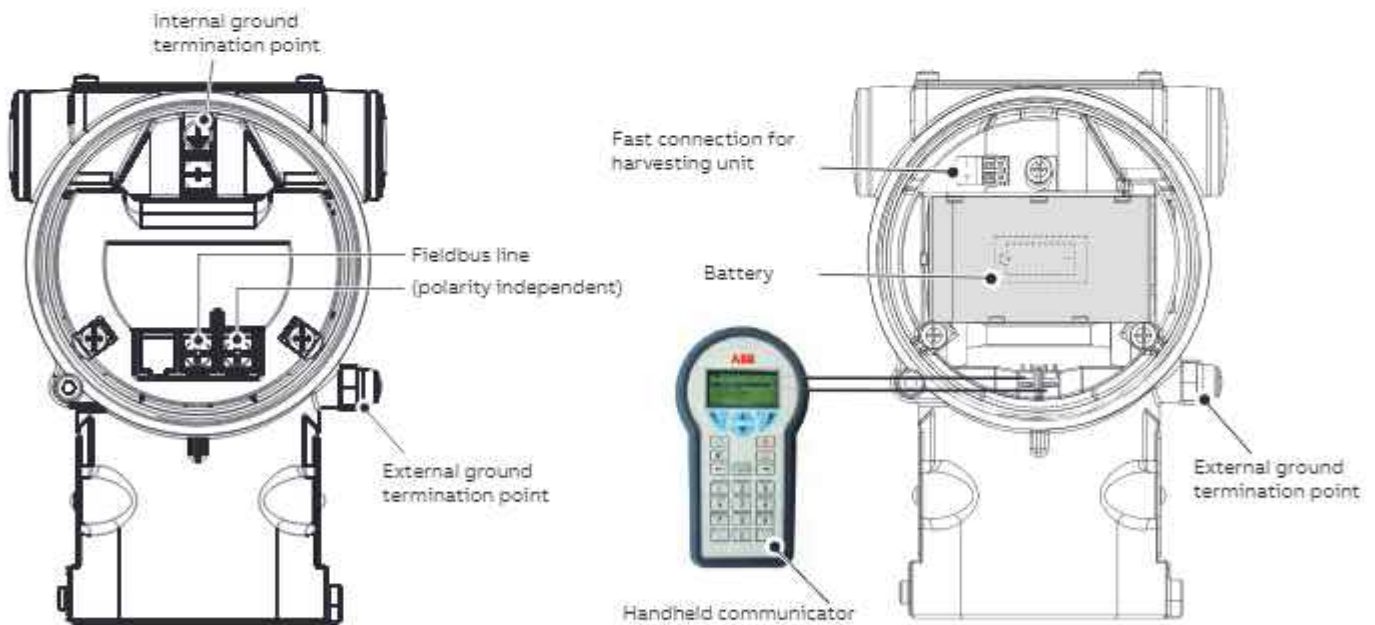
Figure 11 FIELDBUS Versions
